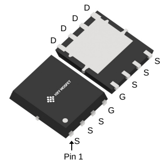
DFN5X6-8L (SO-8FL)
