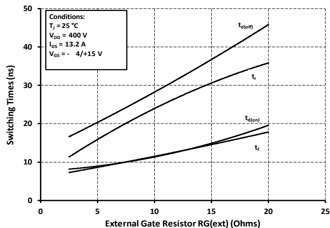
Figure 26. Switching Times vs. R_{G(\text{ext})}
