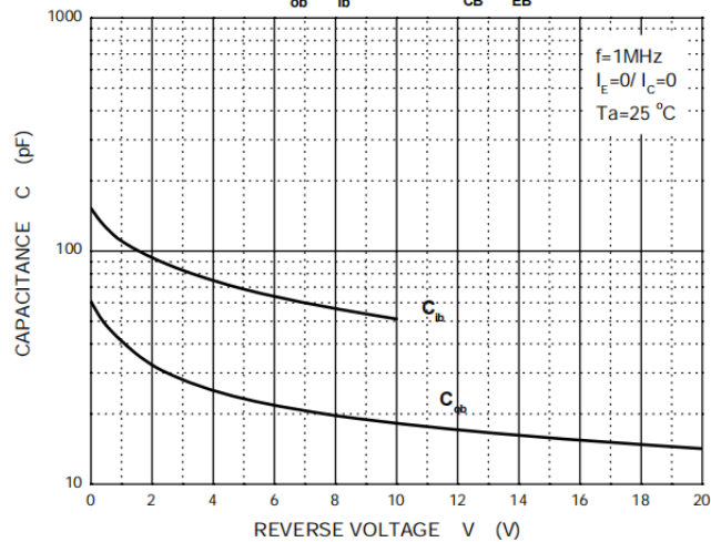
C_{ob}/C_{ib} — V_{CB}/V_{EB}
