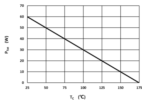
Fig 4: Power Derating
