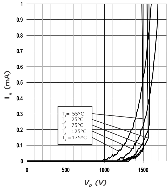
Figure 2. Reverse Characteristics
