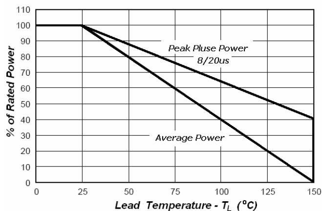
Fig 2. Power Derating
