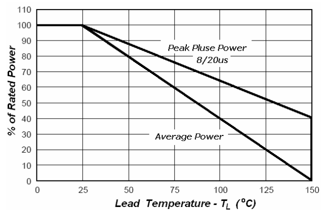
Fig3. Power Derating
