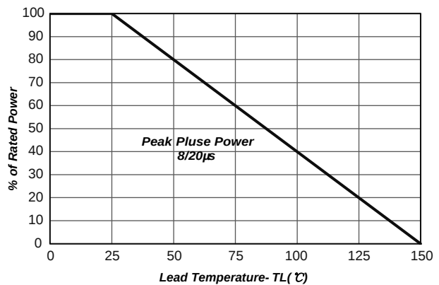
Fig2.Power Derating
