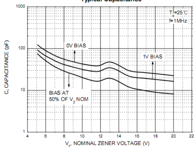
Typical Capacitance
