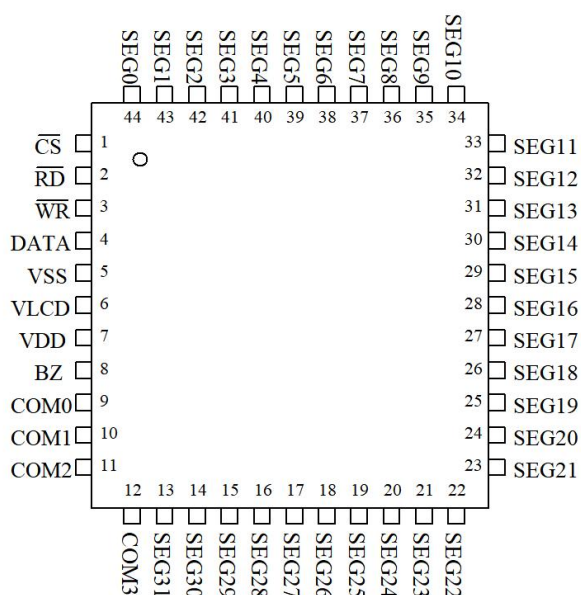
HT1621B LQFP-44
