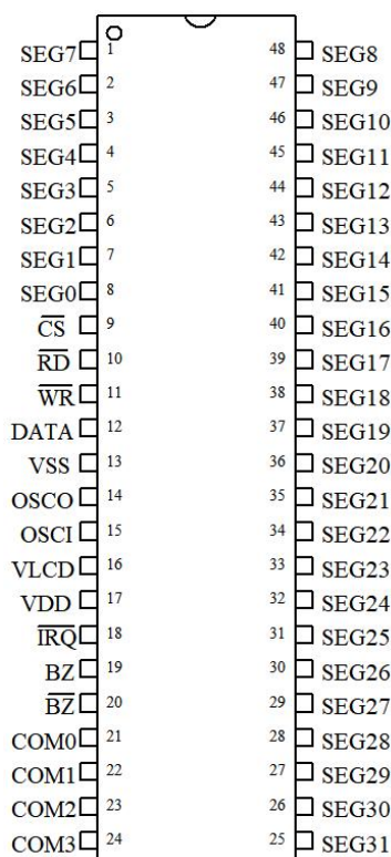
HT1621B SSOP-48
