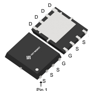
DFN5X6-8L (SO-8-FL-5.9mm)
