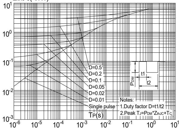
Figure.11: Maximum Effective Transient Thermal Impedance, Junction-to-Case Z_{thj-c} (°C/W)
