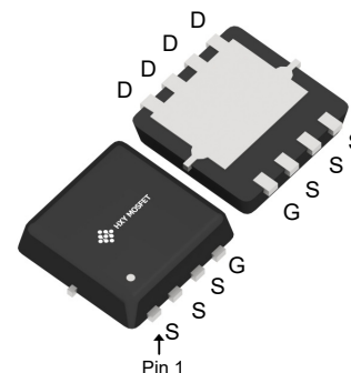
DFN3X3-8L DFN-8(3x3)
