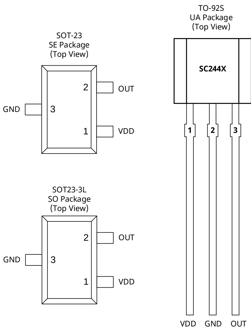
Fig. 2: Terminal Configuration
