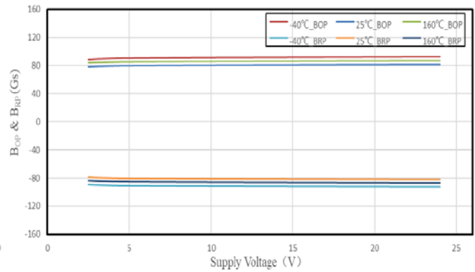
SC2448 B_{OP} & B_{RP} VS. Supply Voltage
