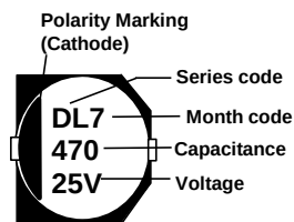
Fig.1 ΦD=4~10mm
