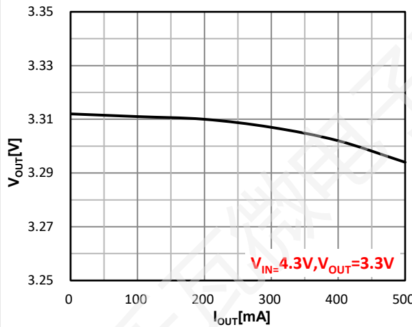
Figure 15. Load Regulation
