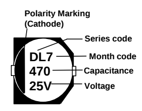
Fig.1 ΦD=4~10mm
