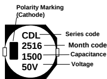
Fig.2 ΦD≥12.5mm
