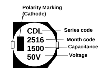
Fig.2 ΦD≥12.5mm
