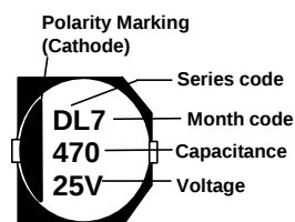
Fig.1 ΦD=4~10mm
