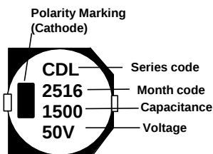
Fig.2 ΦD≥12.5mm
