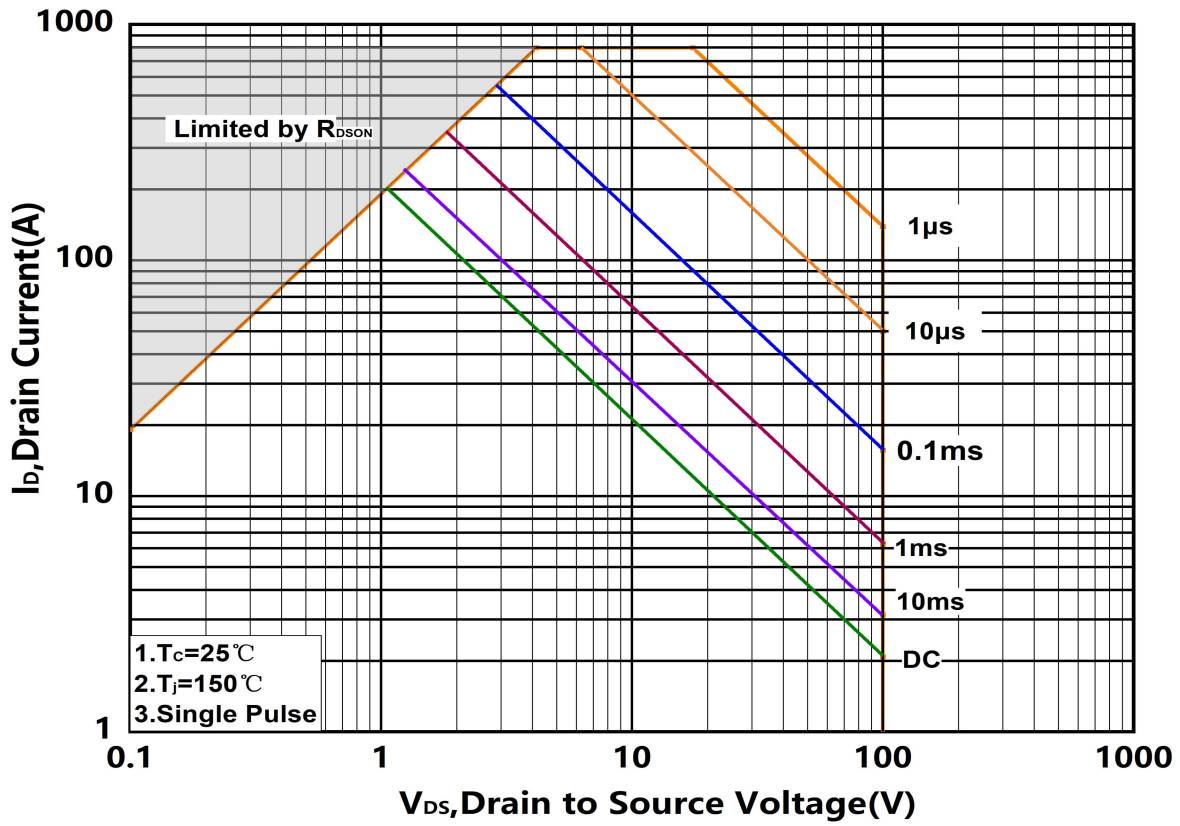
Figure.13 Safe Operating Area
