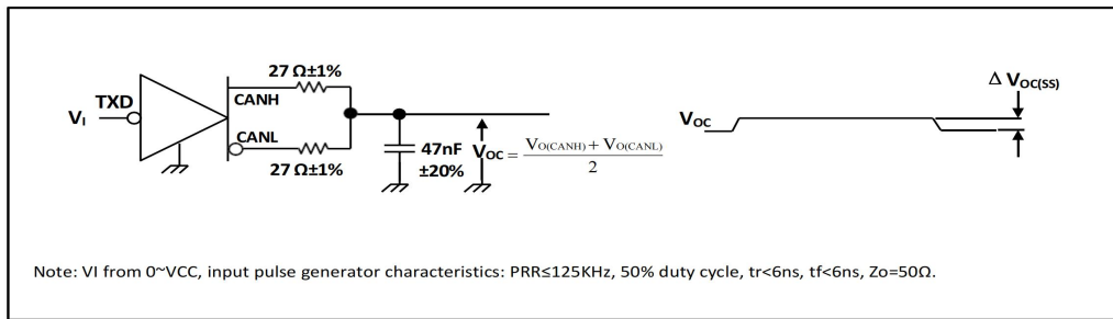
Figure 5-8. Common Mode Output Voltage Test and Waveforms
