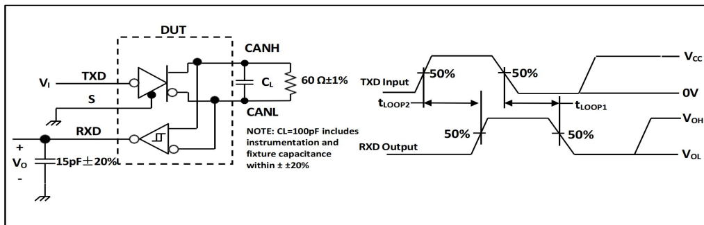
Figure 5-9. t(\text{LOOP}) Test Circuit and Waveforms
