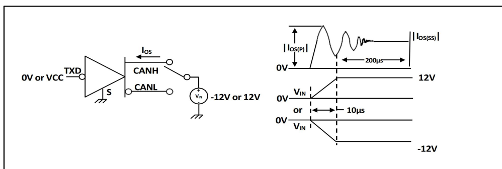
Figure 5-11. Driver Short Circuit Current Test Circuit and Waveforms
