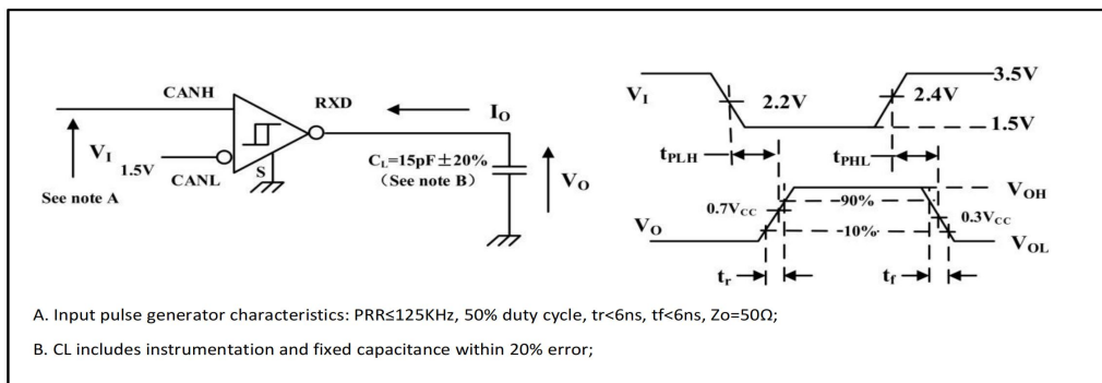
Figure 5-6. Receiver test circuit and voltage waveform
