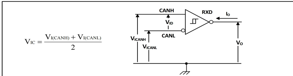
Figure 5-5. Receiver Voltage and Current Definitions
