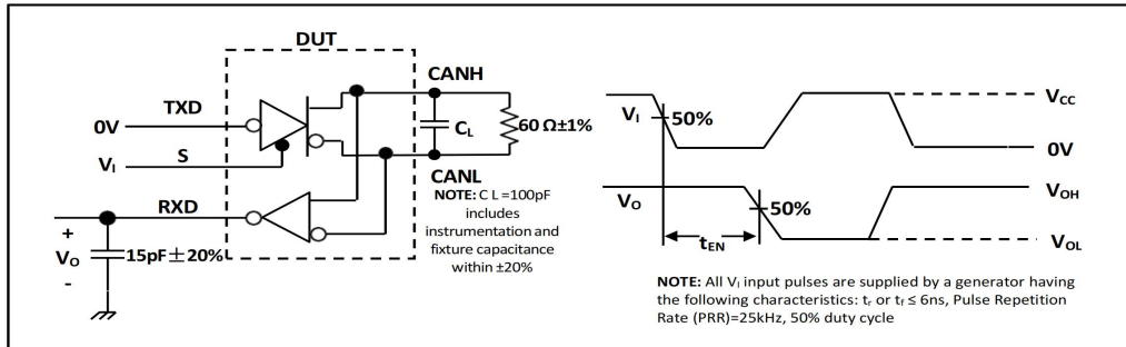
Figure 5-7. t_{EN} Test Circuit and Voltage Waveforms
