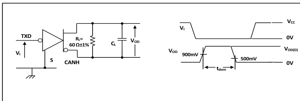
Figure 5-10. Revealed Timeout Test Circuit and Waveforms
