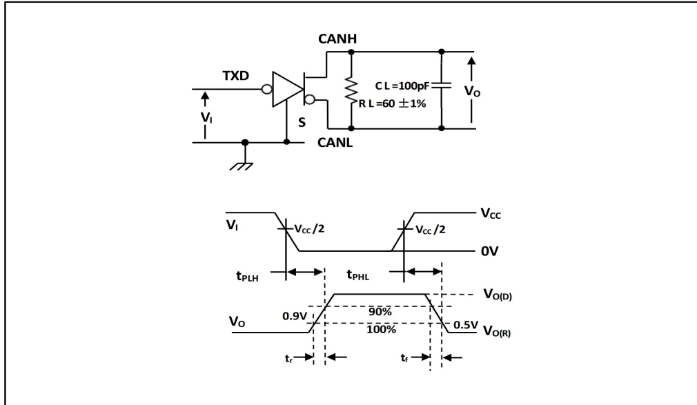
Figure 5-4. Driver Test Circuit and Voltage Waveforms
