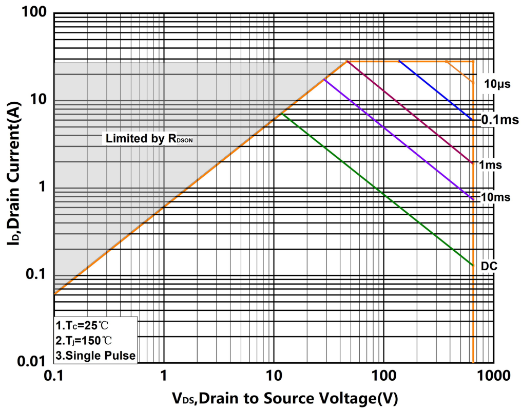
Figure.11 Safe Operating Area
