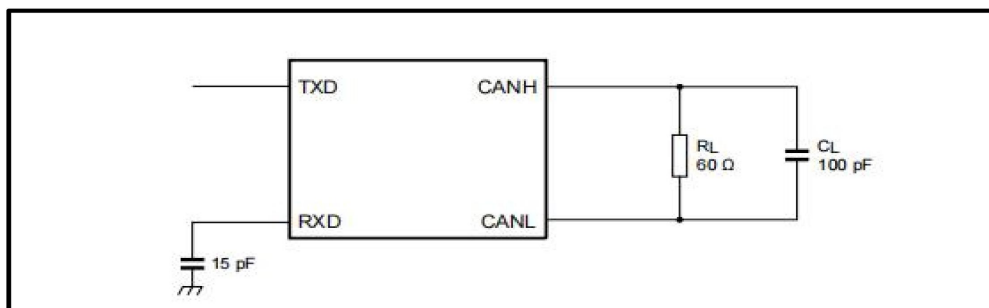
Figure 5. CAN transceiver timing test circuit
