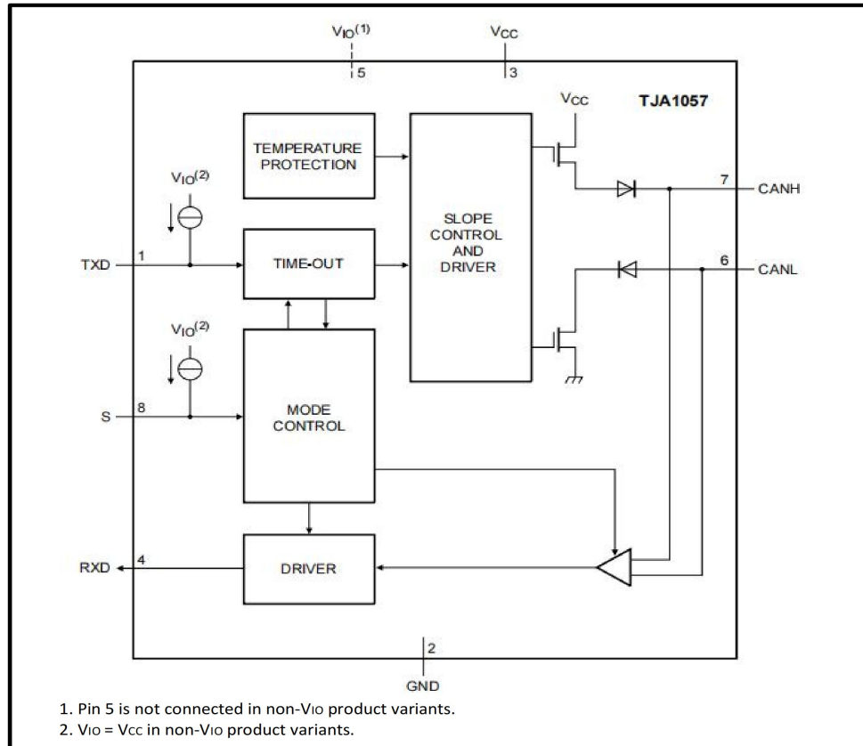
Figure 1. Block diagram
