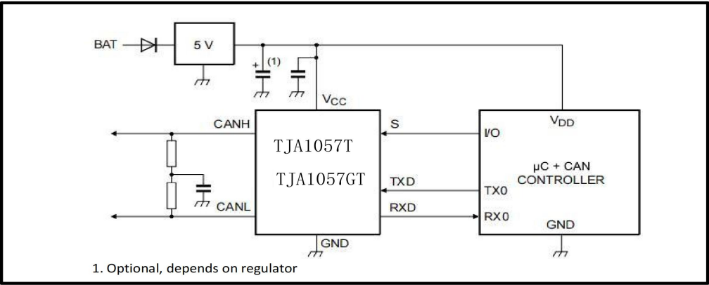
Figure 4. Typical TAJ1057 application with a 5 V microcontroller (non- V_{IO} variants)
