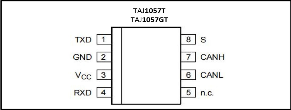
Figure 2. Pin configuration diagrams
