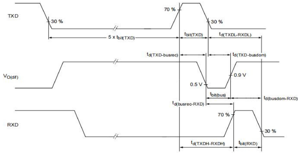
Figure 3. CAN transceiver timing diagram according to ISO 11898-2:2024
