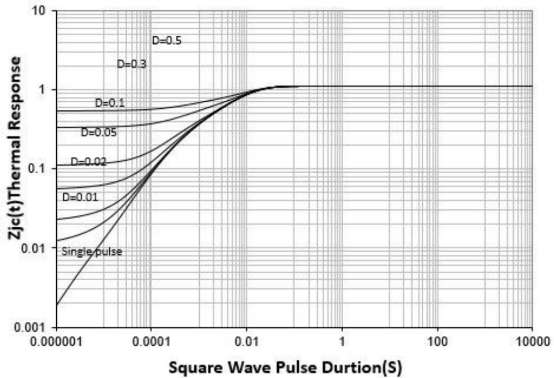
Figure 10: Maximum Transient Thermal Impedance (Note 5)
