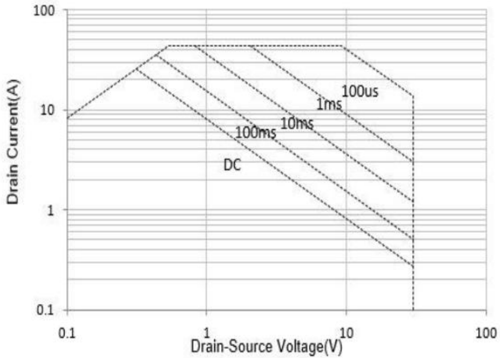
Figure.9 Maximum Forward Biased Safe Operating Area
