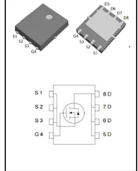
View and Internal Schematic Diagram PDFN5*6-8L
