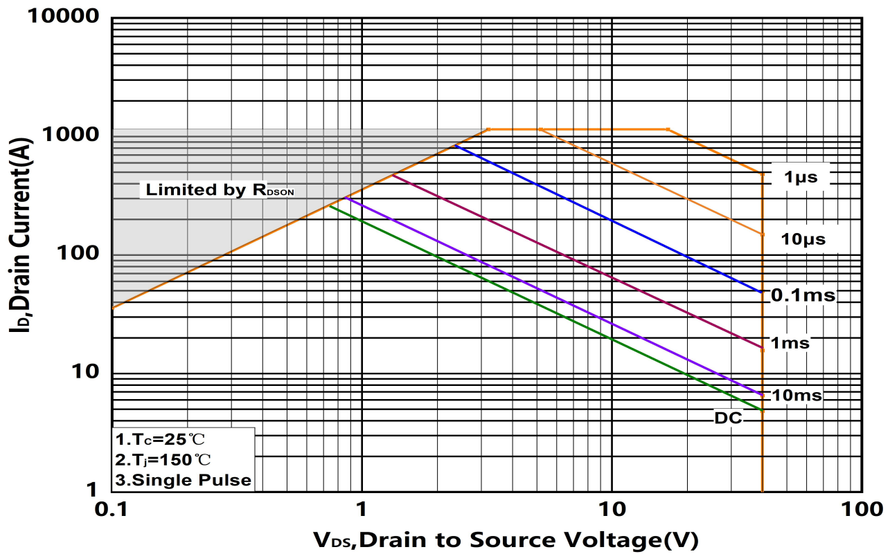
Figure.13 Safe Operating Area
