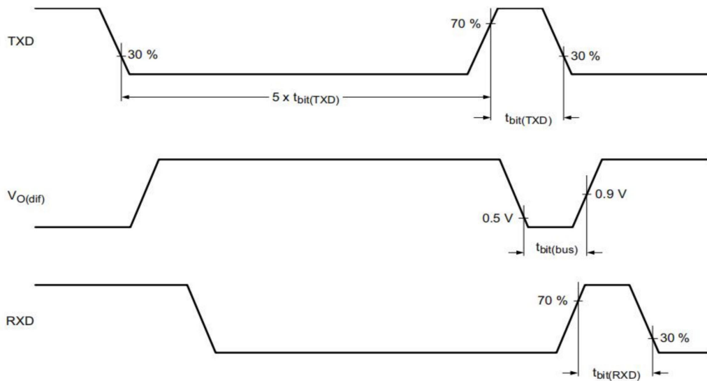
Figure 4. CAN FD timing definitions according to ISO 11898-2:2016
