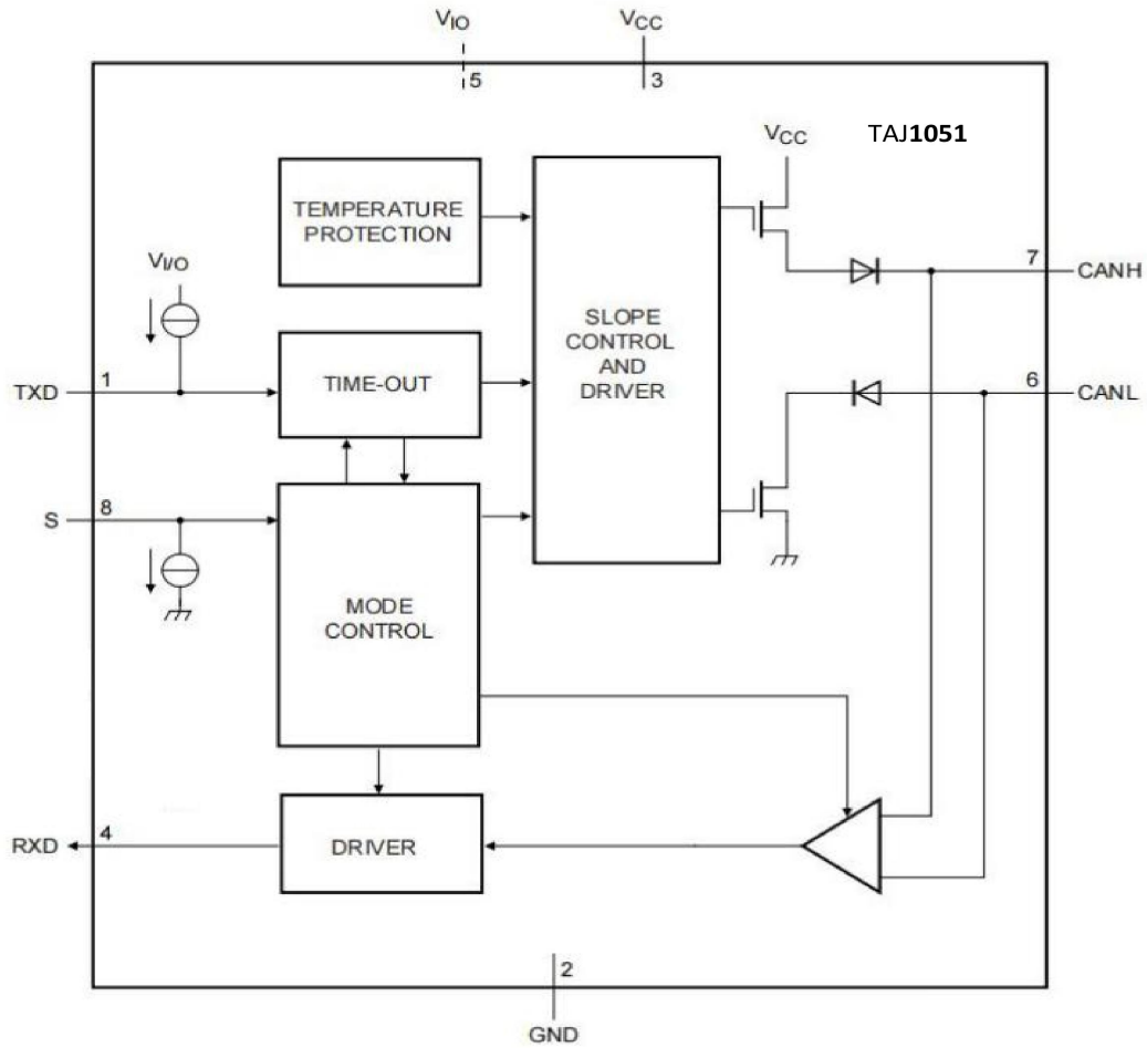
Figure 1. Block diagram
