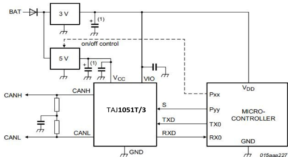
Figure 5. Typical application of the TAJ1051T/3 with 3V system
