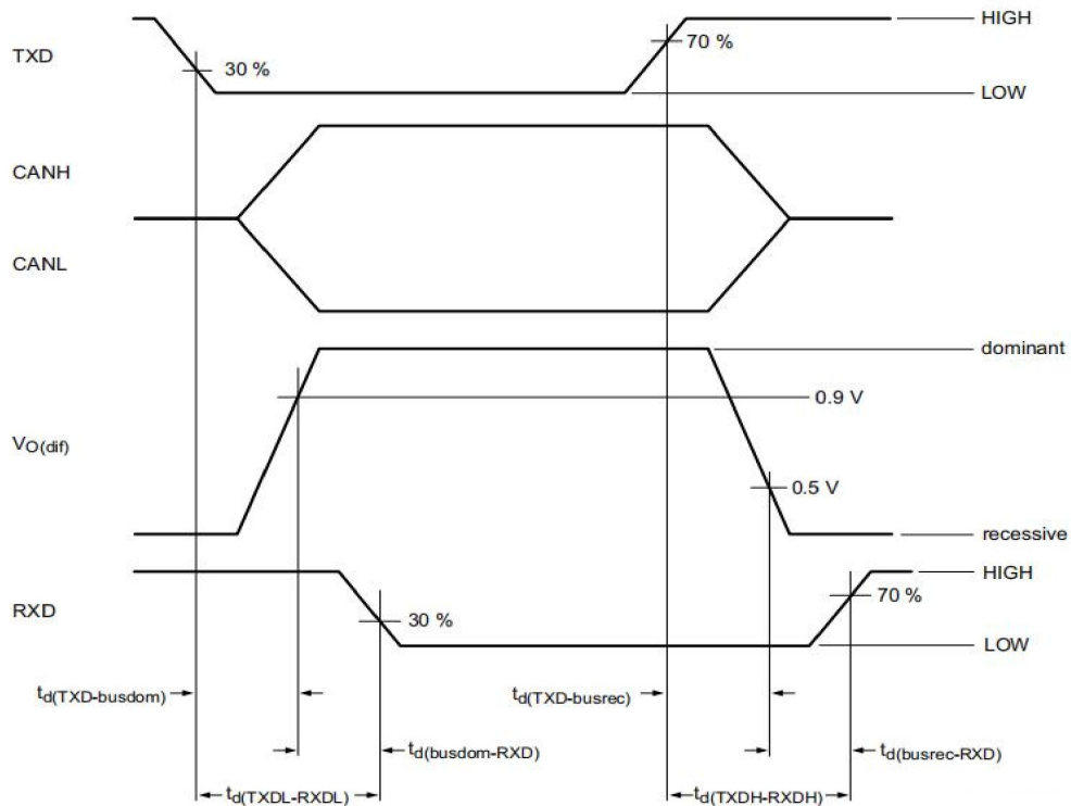
Figure 3. CAN transceiver timing diagram
