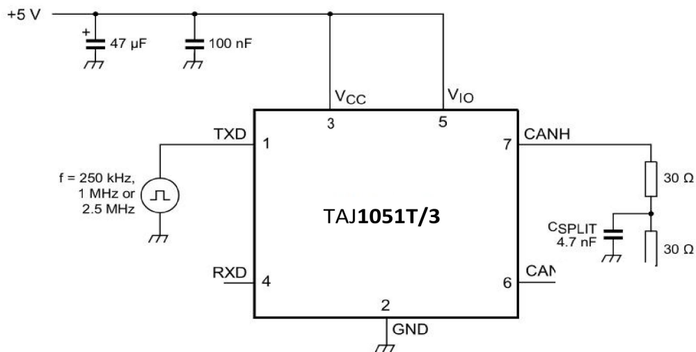
Figure 7. Test circuit for measuring transceiver driver symmetry
