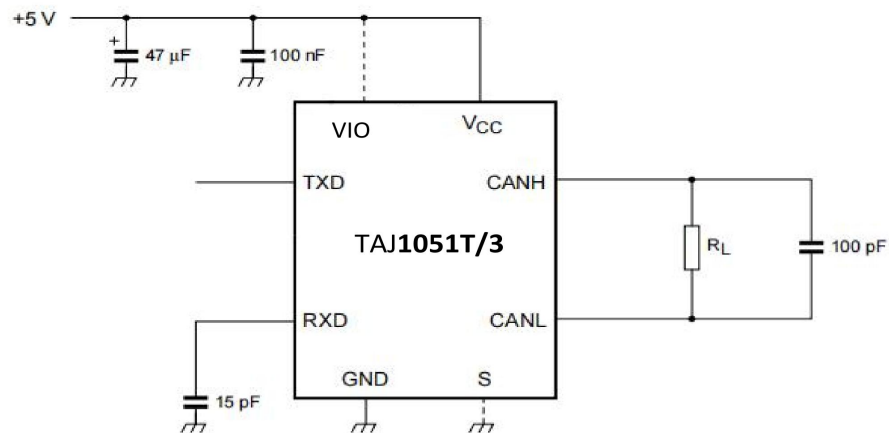
Figure 6. Timing test circuit for CAN transceiver
