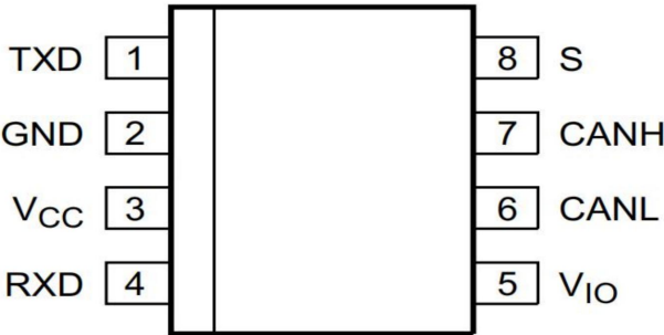
(Top View) Figure 2. Pin configuration diagrams
