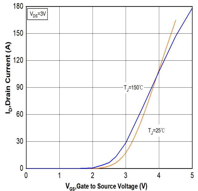
Figure.2 Transfer Characteristic for Various Junction Temperatures
