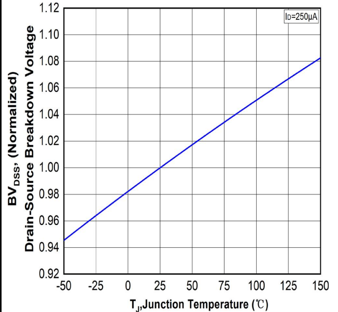
Figure.6 Typical Breakdown Voltage vs Junction Temperature
