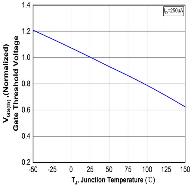
Figure.5 Typical Threshold Voltage vs Junction Temperature
