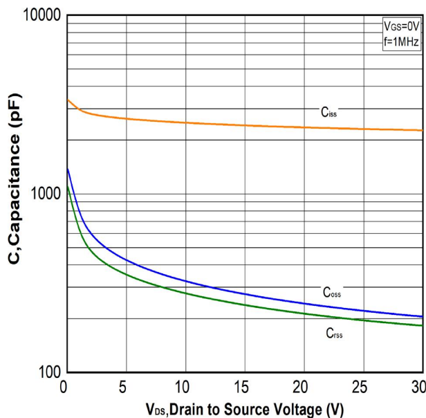
Figure.7 Typical Capacitance vs Drain to Source Voltage
