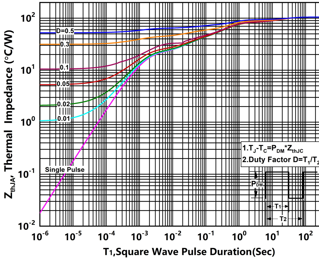
Figure.11 Transient Thermal Impedance (Junction - Case)
