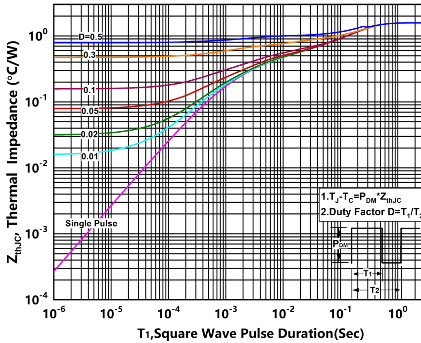
Figure.12 Transient Thermal Impedance (Junction - Case)
