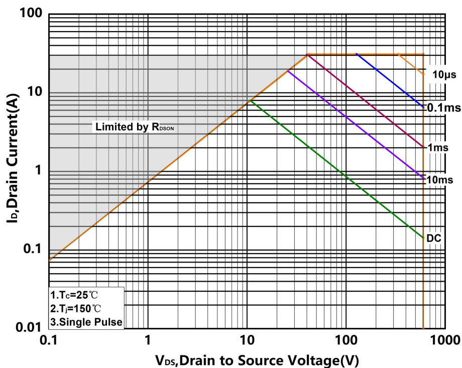
Figure.12 Safe Operating Area
