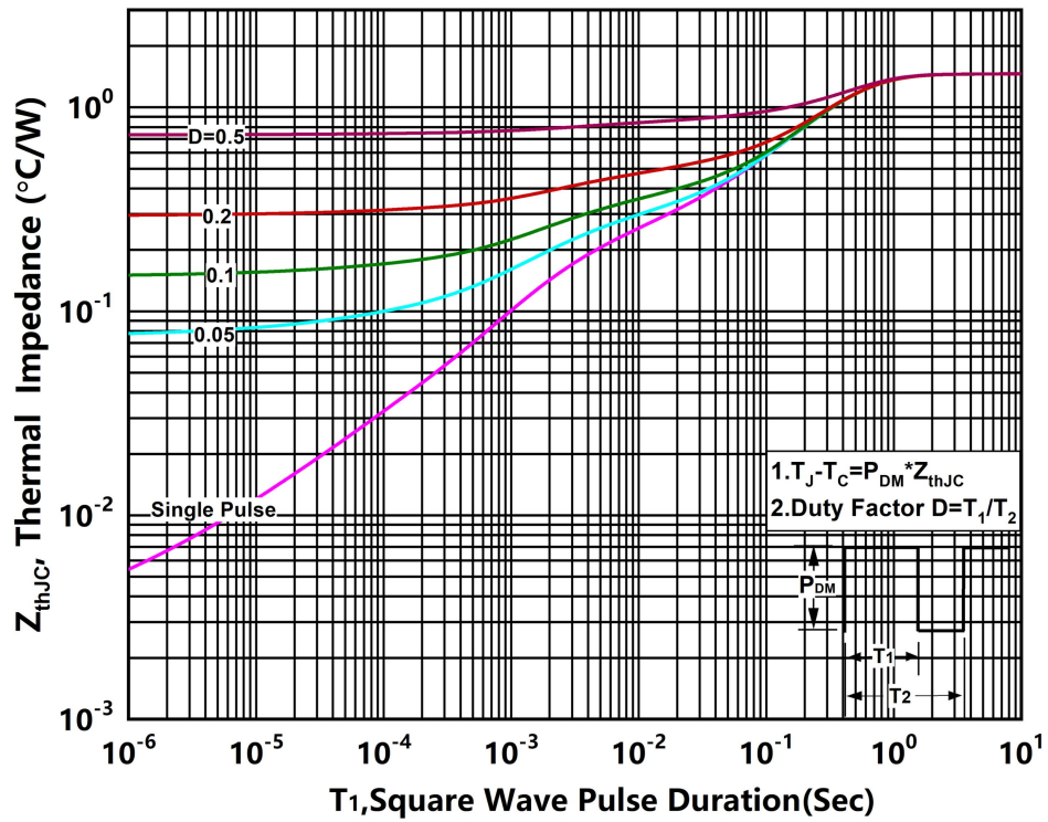
Figure.13 Transient Thermal Impedance (Junction - Case)
