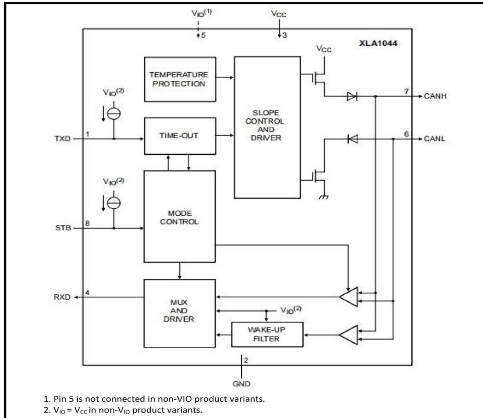
Figure 1. Block diagram
