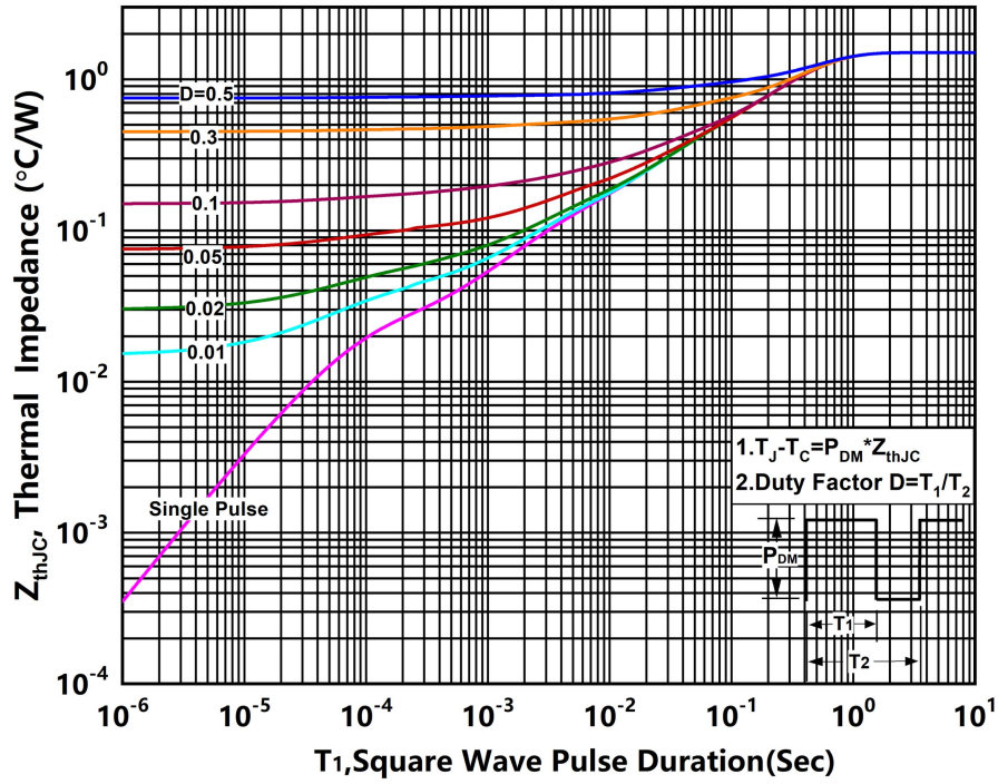
Figure.12 Transient Thermal Impedance (Junction - Case)
