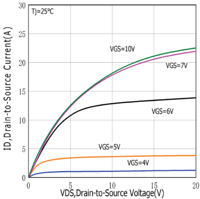
Figure.1 Output Characteristics
