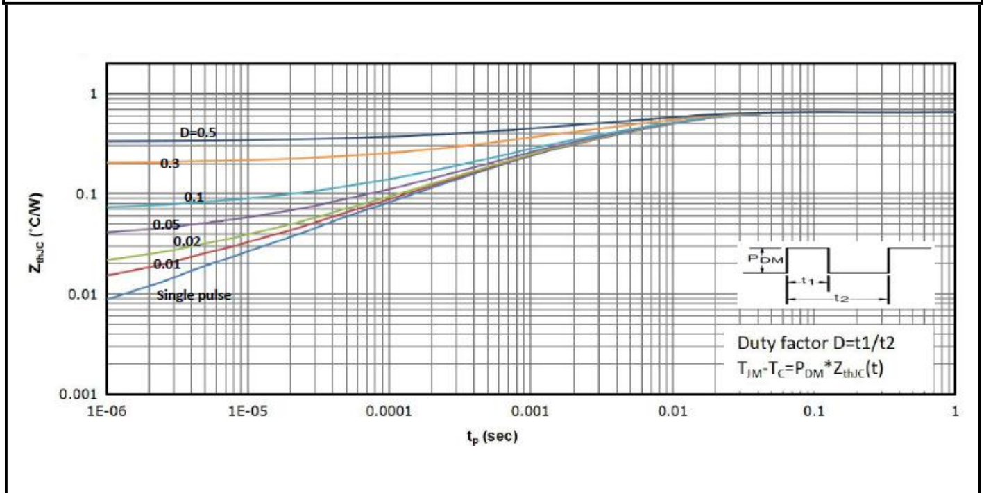
Figure.14 Maximum Effective Thermal Impedance, Junction to Case
