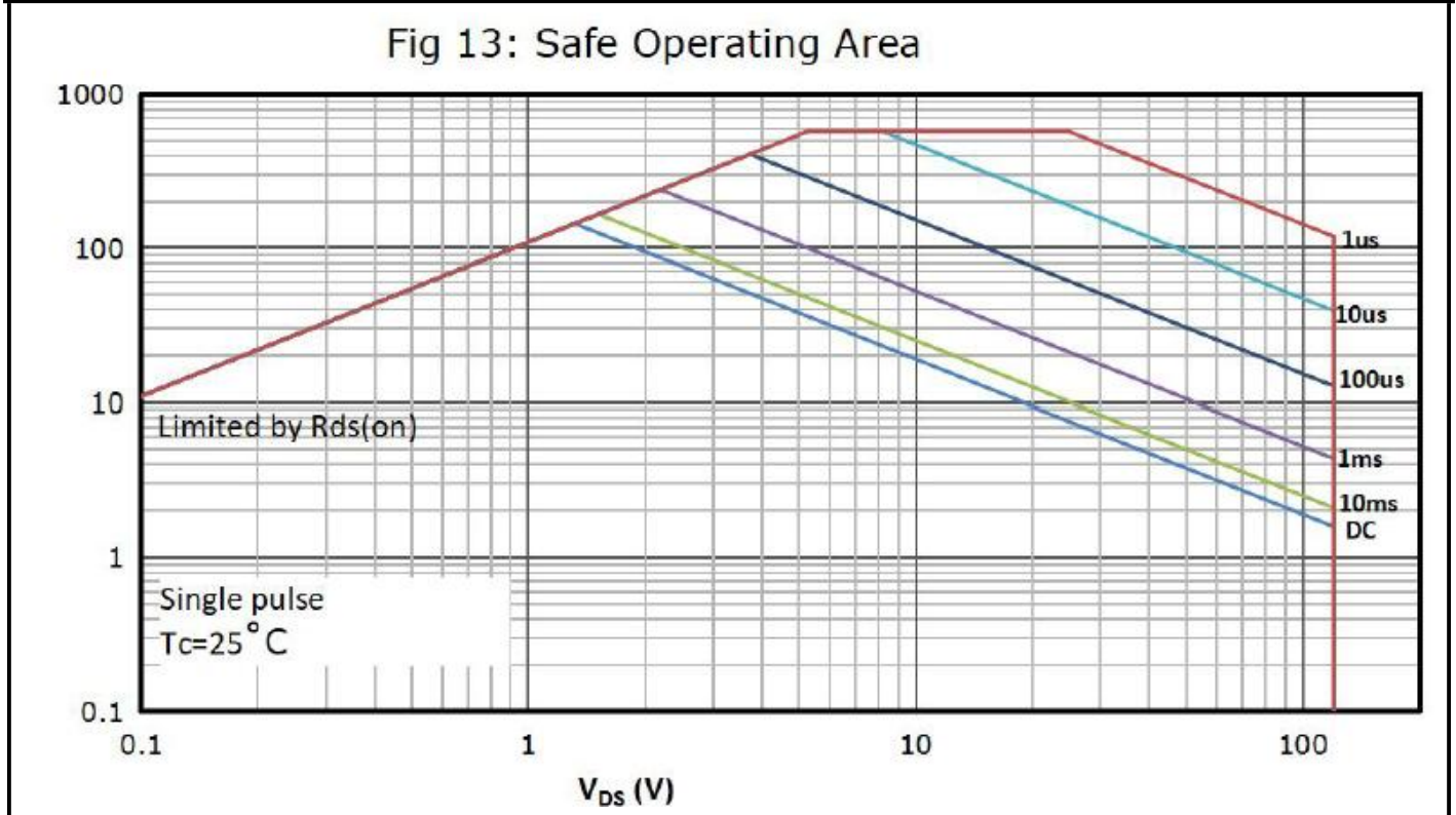
Figure.13 Safe Operating Area
