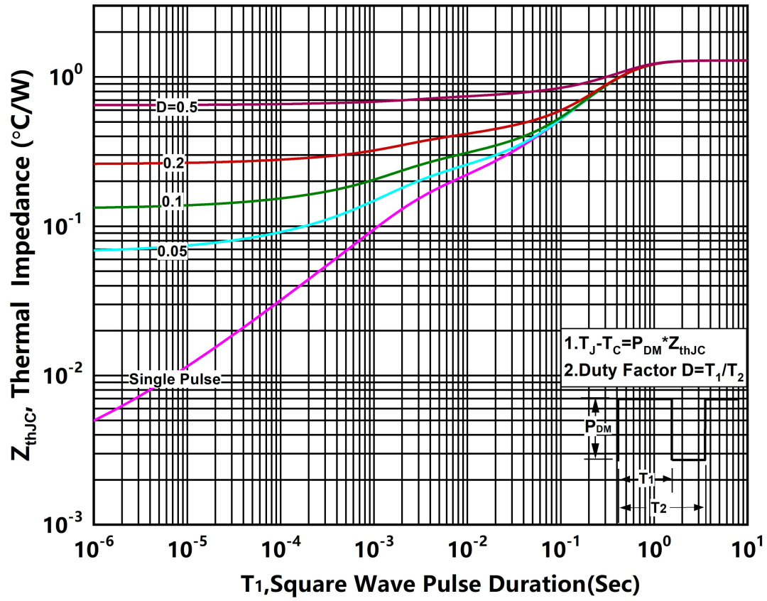
Figure.12 Transient Thermal Impedance (Junction - Case)
