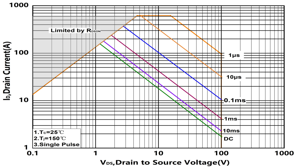
Figure.13 Safe Operating Area
