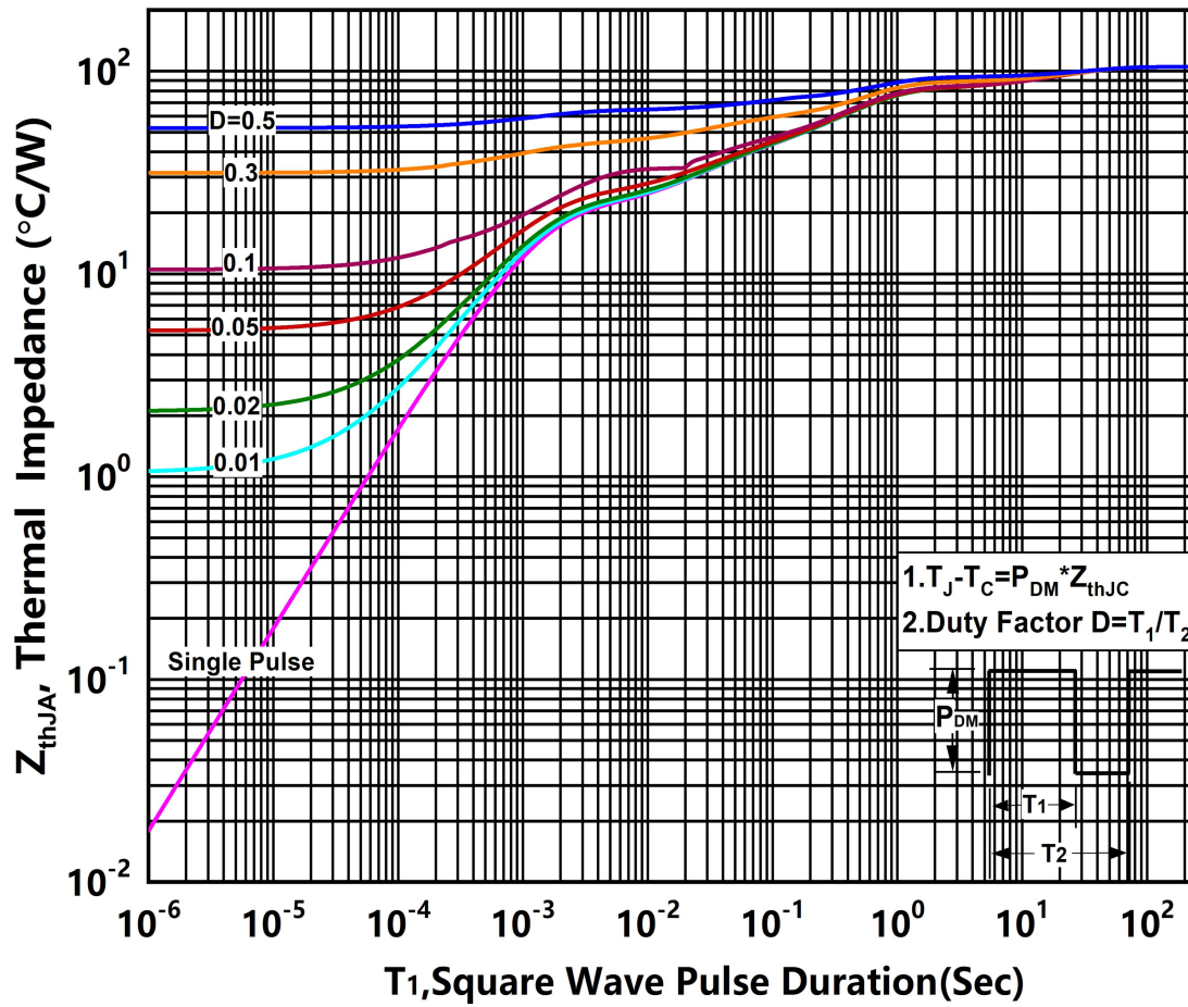
Figure.13 Transient Thermal Impedance (Junction - Case)
