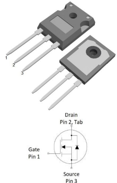
View and Internal Schematic Diagram TO-247-3L
