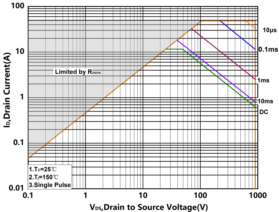
Figure.11 Safe Operating Area
