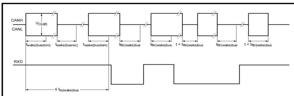
Figure 3. Wake-up timing
