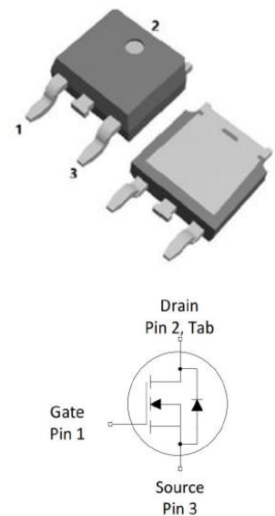
View and Internal Schematic Diagram TO-252-2L
