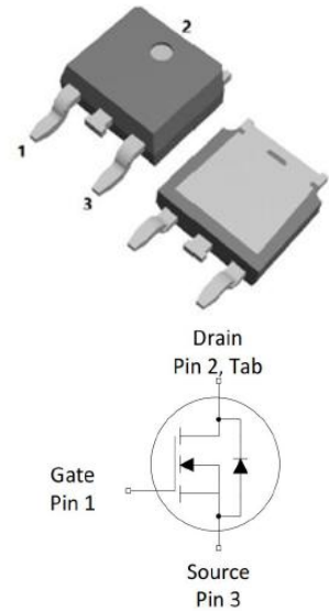
View and Internal Schematic Diagram TO-252-2L
