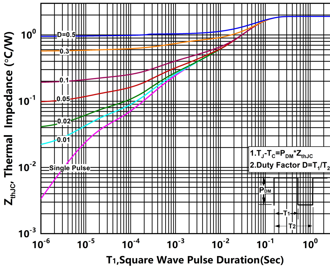
Figure.12 Transient Thermal Impedance (Junction - Case)
