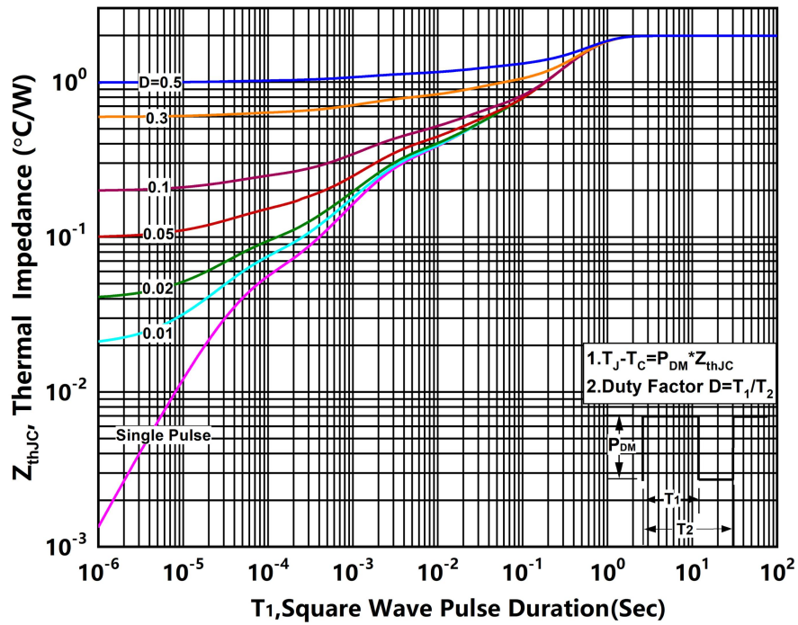
Figure.13 Transient Thermal Impedance (Junction - Case)
