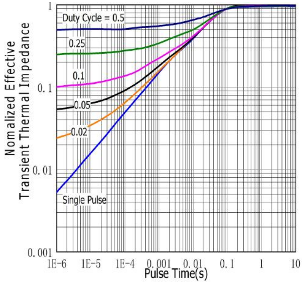
Figure.13 Maximum Effective Thermal Impedance , Junction to Case
