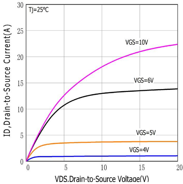
Figure.1 Output Characteristics
