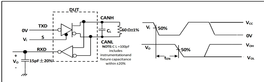
Figure 6-7. t_{EN} Test Circuit and Voltage Waveforms
