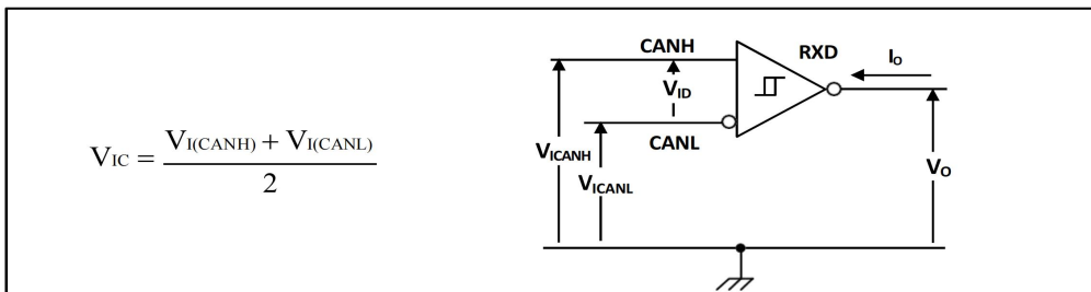
Figure 6-5. Receiver Voltage and Current Definitions
