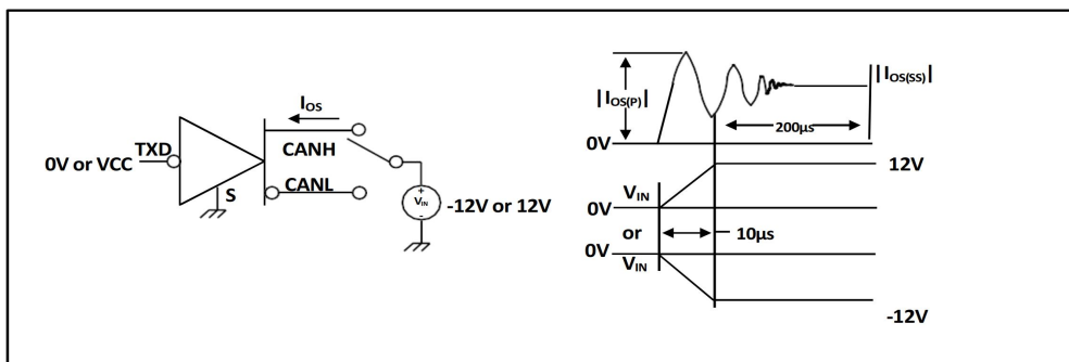
Figure 6-11. Driver Short Circuit Current Test Circuit and Waveforms
