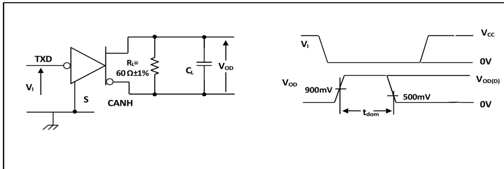
Figure 6-10. Revealed Timeout Test Circuit and Waveforms
