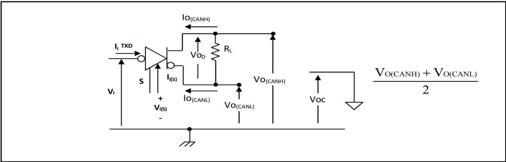
Figure 6-1. Driver Voltage, Current Test Definitions
