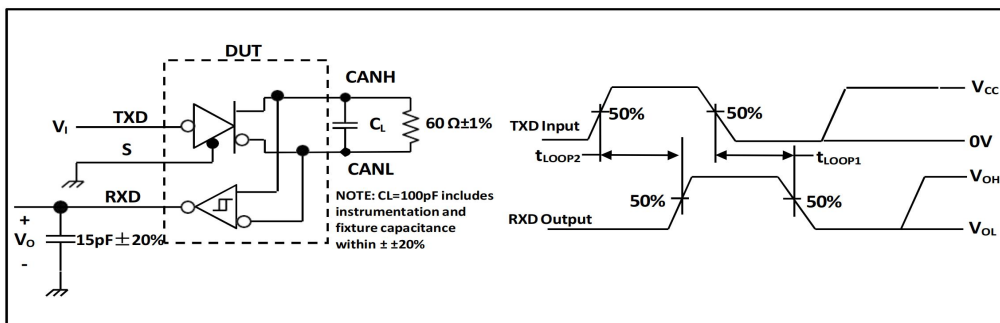
Figure 6-9. t_{(LOOP)} Test Circuit and Waveforms
