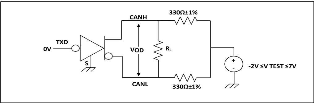
Figure 6-3. Driver VOD Test Circuit
