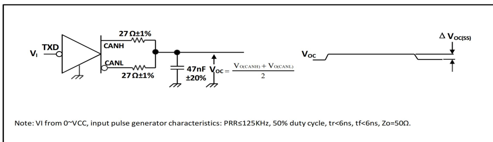
Figure 6-8. Common Mode Output Voltage Test and Waveforms
