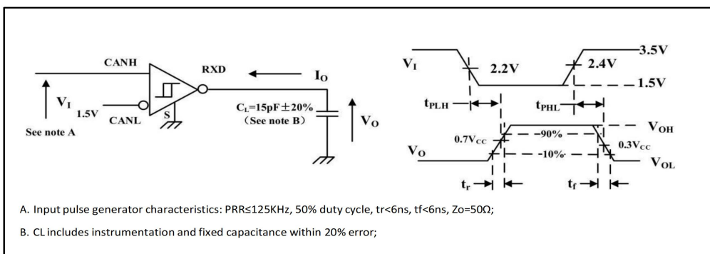
Figure 6-6. Receiver test circuit and voltage waveform
