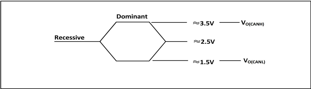
Figure 6-2. Bus Logic Voltage Definition
