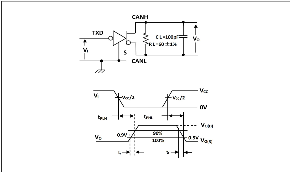
Figure 6-4. Driver Test Circuit and Voltage Waveforms
