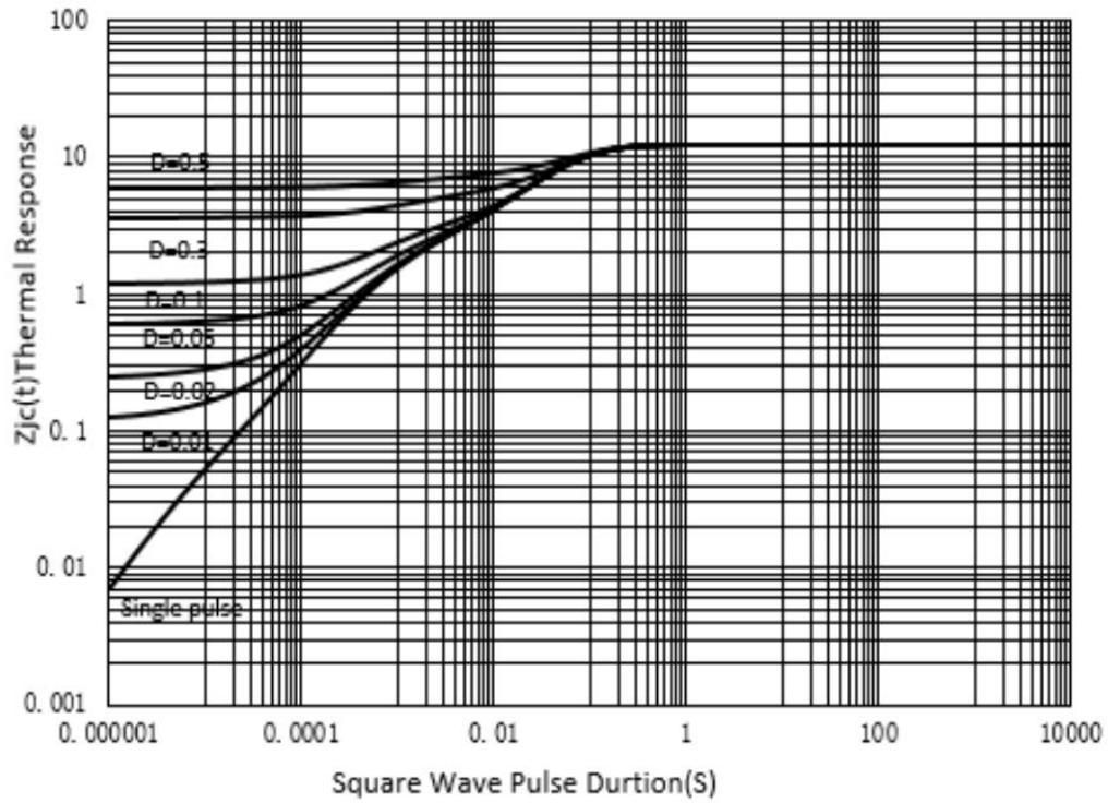
Figure 11: Maximum Transient Thermal Impedance
