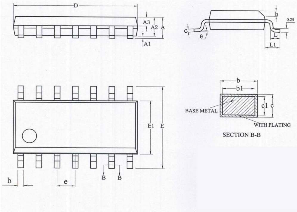
SOP14
