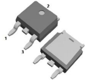
View and Internal Schematic Diagram TO-252-2L
