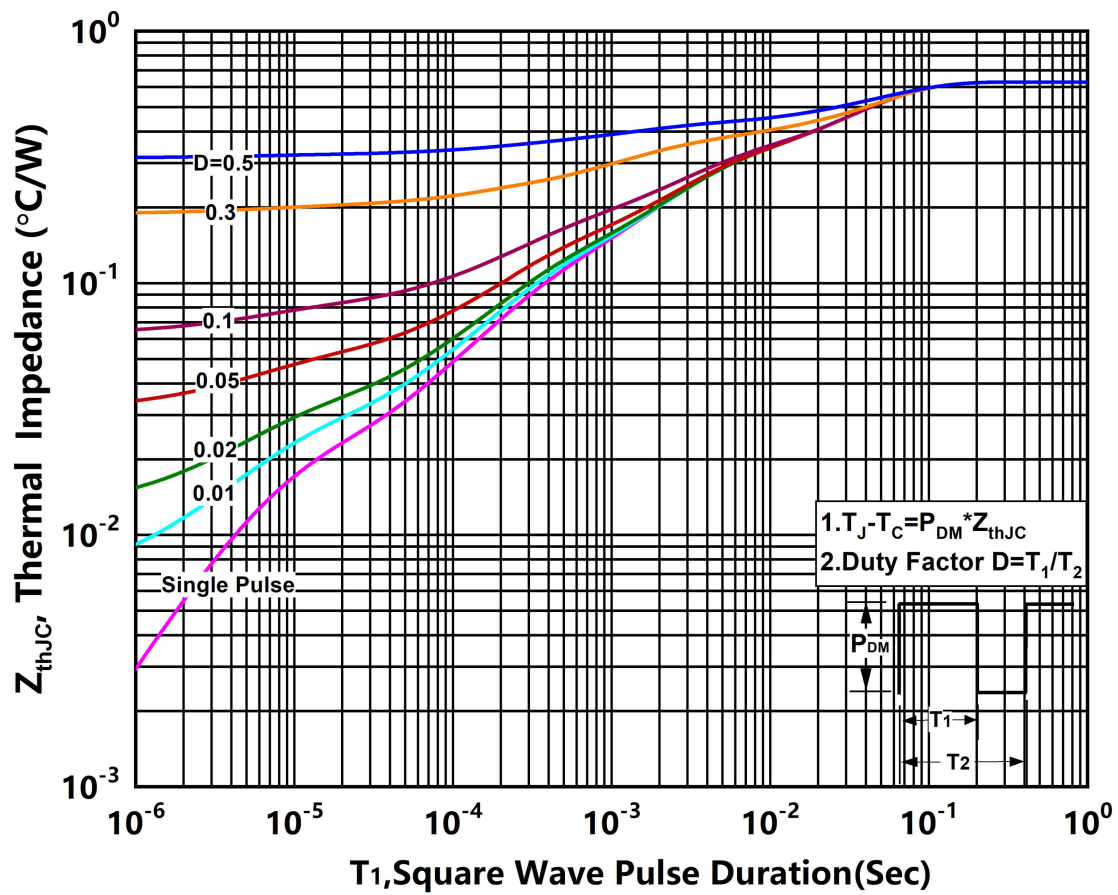
Figure.12 Transient Thermal Impedance (Junction - Case)
