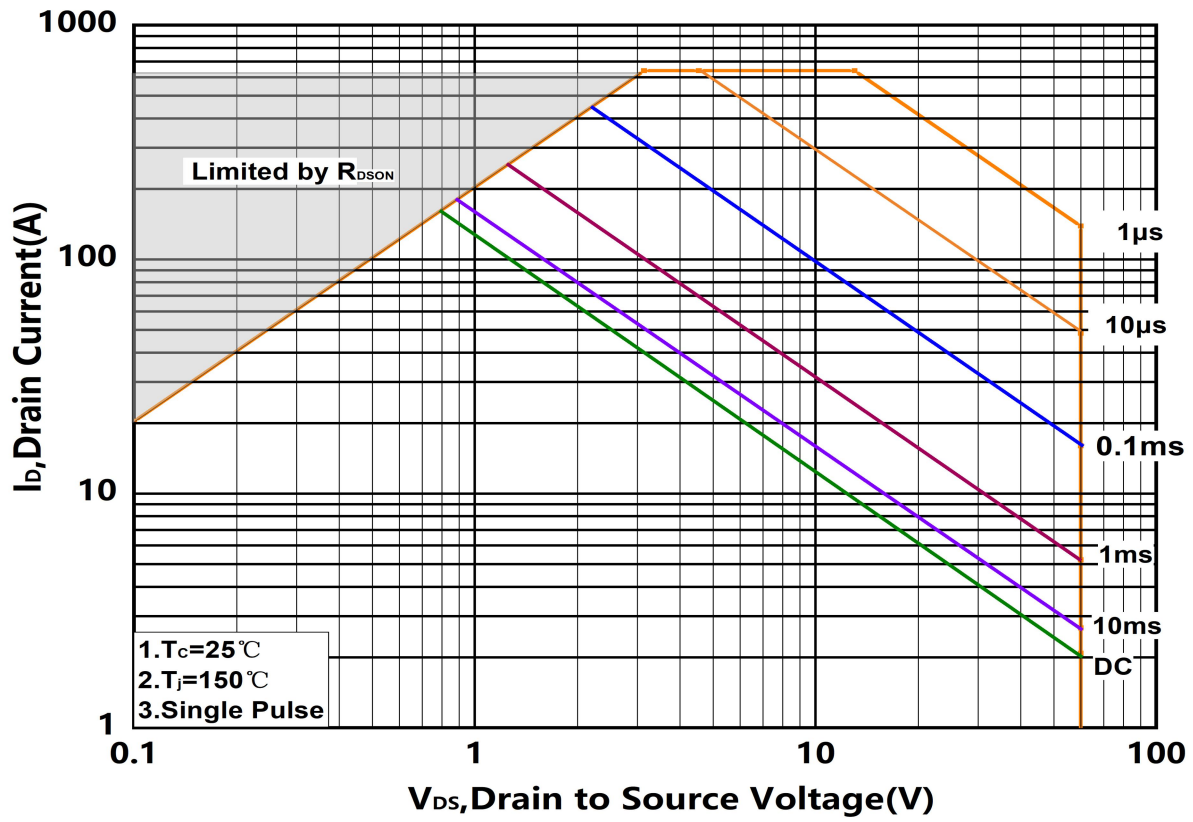
Figure.13 Safe Operating Area
